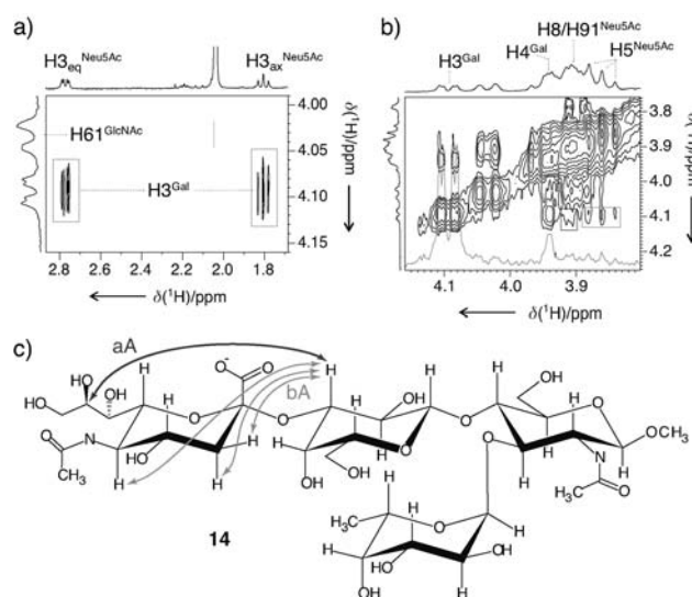
Figure 2. a,b) Portions of the trNOESY spectrum (500 MHz, \text{D}_2\text{O} ) of 0.25 mM \text{sLe}^x 14 in the presence of 1.2 \text{ mg mL}^{-1} NV VLPs; a 13:1 ratio of ligand to binding sites is observed if one assumes 180 binding sites per VLP. T = 298 \text{ K} ; mixing time: 250 ms. c) Interglycosidic trNOEs across the 2,3-glycosidic linkage between \text{H3}^{\text{Gal}} and \text{H3}_{\text{ax}}^{\text{Neu5Ac}}/\text{H3}_{\text{eq}}^{\text{Neu5Ac}} and \text{H5}^{\text{Neu5Ac}} (light gray arrows corresponding to light gray boxes in (a,b)) and between \text{H3}^{\text{Gal}} and \text{H8}^{\text{Neu5Ac}} (dark gray arrow corresponding to the dark gray box in (b)).
